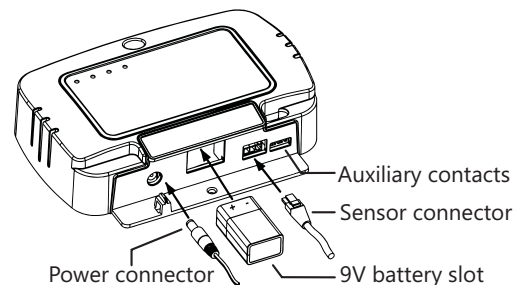
Figure 1. Connection Locations on Bottom of Alarm Unit
