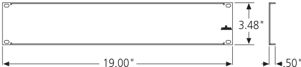
2RU Standard Blank Panel
