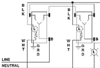
3-Way Pilot Light
