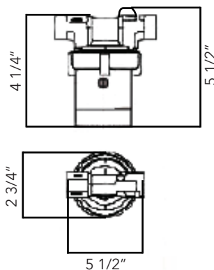
UltraCirc Pump Housing (Union with Ball Valve & Check Valve)
