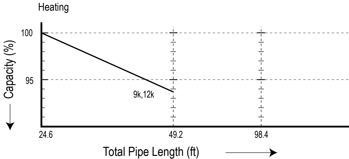
Figure 20: LS090HXV, LS120HXV Heating Coefficient Factor.
