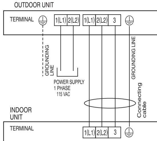
Figure 23: Terminal Block Wiring Diagram LS090HXV2, LS120HXV2.
