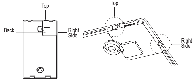
Figure 36: Attaching the Wall Plate.
