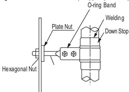
Figure 276: One-Point Down-Stop Support (>441 lbs.).
