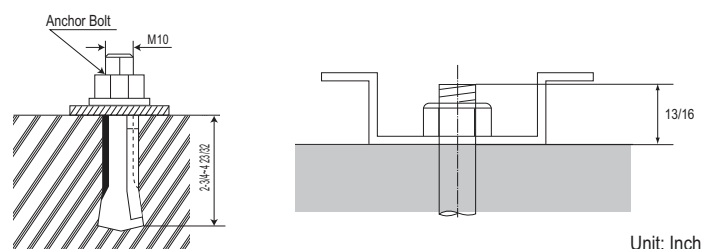
Figure 255: Close up of Bolt Attachment.
