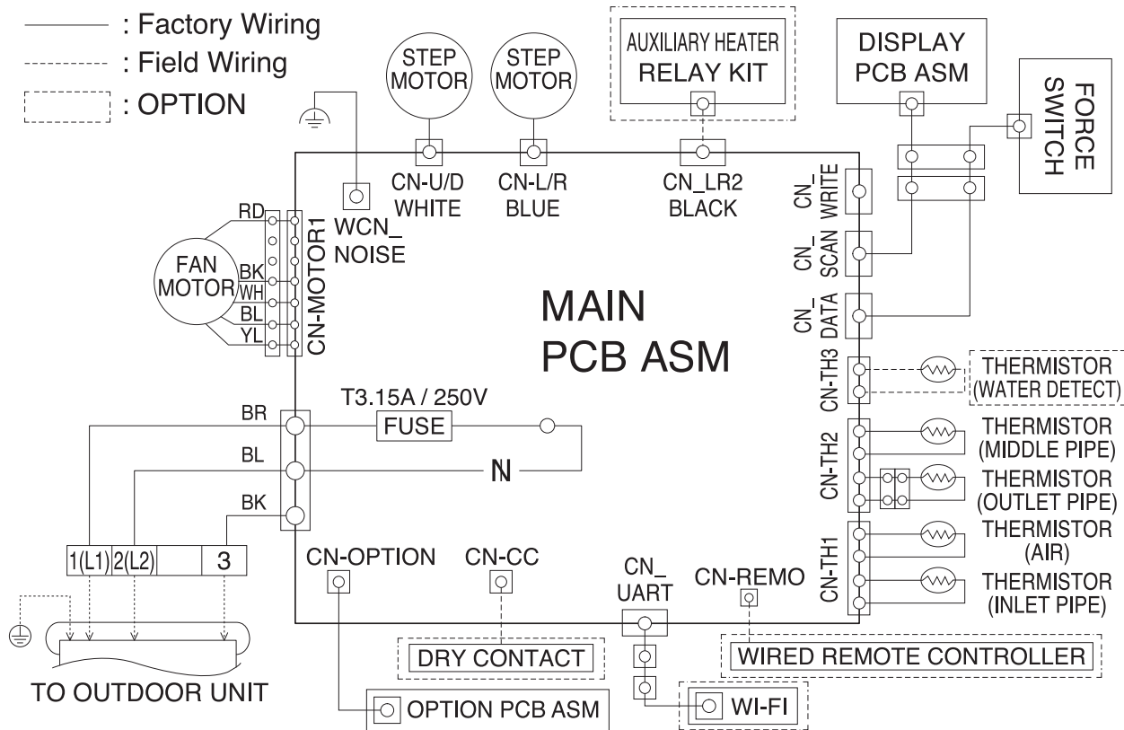
Figure 88: Multi F Standard Wall-Mounted LSN180HSV4 Indoor Unit Wiring Diagram.
