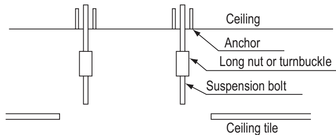
Figure 201: Installing the Hanging Bolt in the Ceiling.
