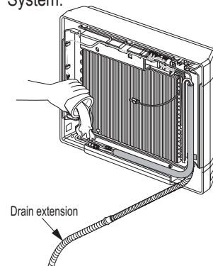
Figure 60: Checking the Drainage System.
