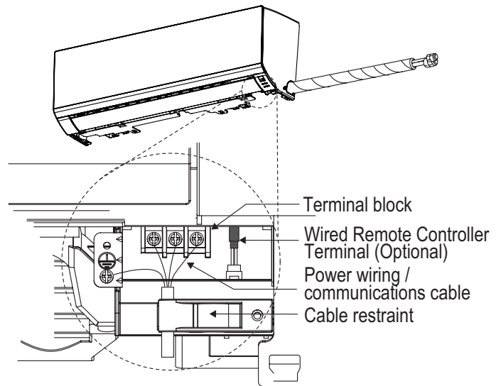
Figure 28: Connecting the Power Wiring / Communications Cable.
