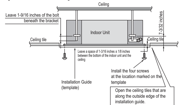
Figure 202: Installation Diagram.
