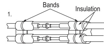
Figure 102: Insulating the Piping.
