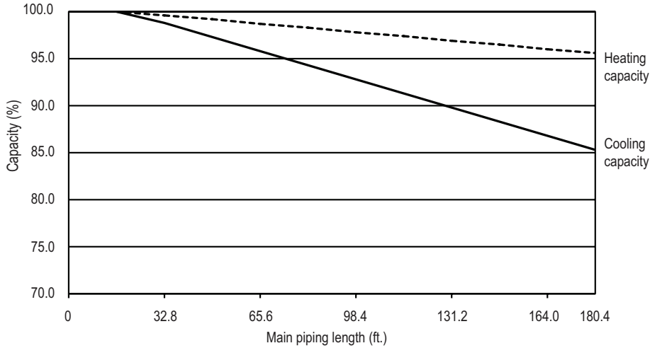
Figure 247: Multi F MAX Outdoor Unit to Branch Distribution Unit Refrigerant Line Length Derate Chart.
