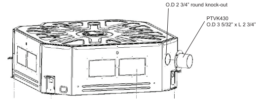
Figure 216: PTVK430 Ventilation Kit.
