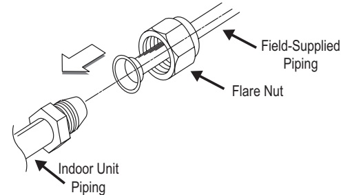
Figure 289: Flare Connection, Side View.
