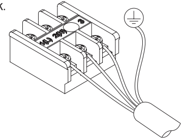
Figure 303: Close up of the Indoor Unit Terminal Block.
