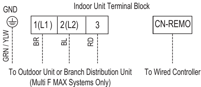
Figure 112:Wired Controller Connection on the Indoor Unit Terminal Block—LSN090HSV4 and LSN120HSV4 models.
