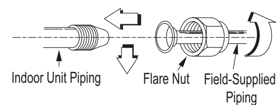
Figure 290: Using the Torque Wrench.
