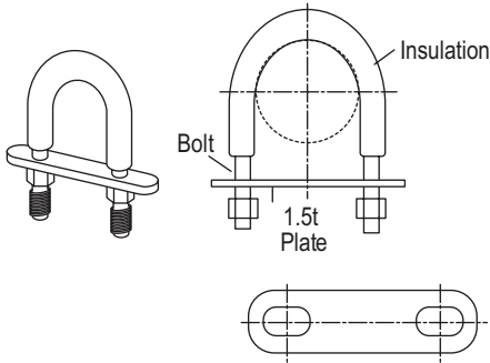
Figure 271: U-Bolt Support with Insulation.
