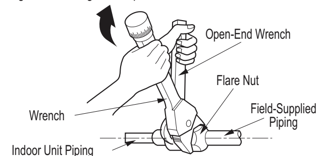
Figure 290: Using the Torque Wrench.
