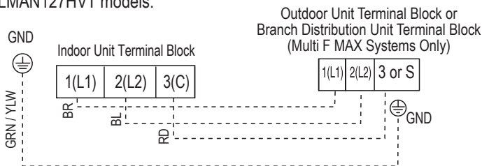
Figure 29: Simplified View of Indoor Unit to Outdoor Unit / Branch Distribution Unit Terminal Connections—LMAN097HVT and LMAN127HVT models.
