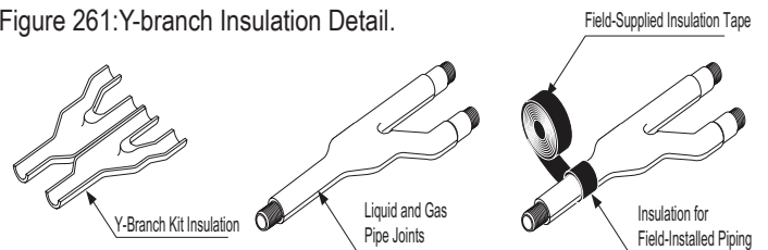
Figure 261: Y-branch Insulation Detail.
