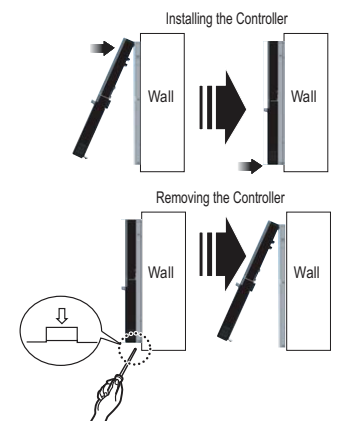
Figure 120: Installing / Removing the Controller.
