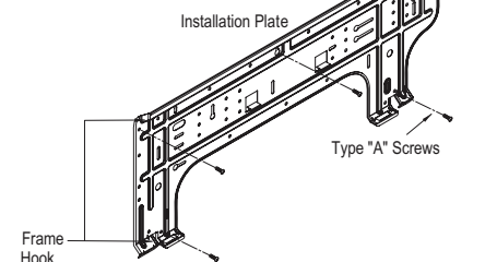
Figure 15: Installation Plate for LMAN187HVT Units.
