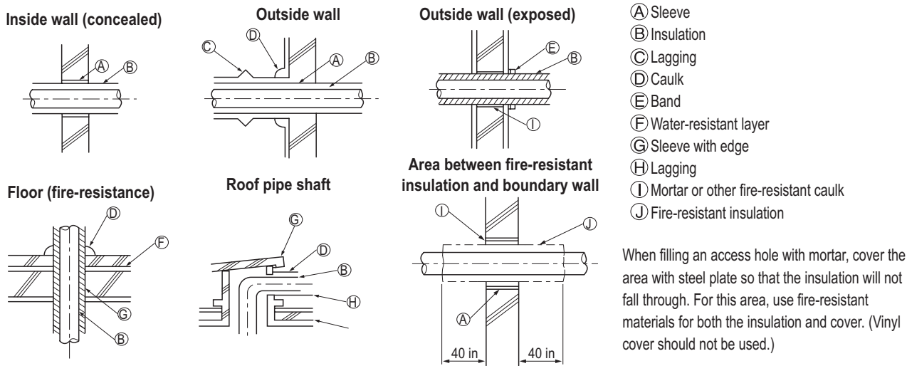
Figure 278: Pipe Sleeve Options.
