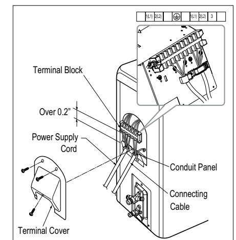
Figure 48: LSU240HEV1 Outdoor Unit Electrical Connection.
