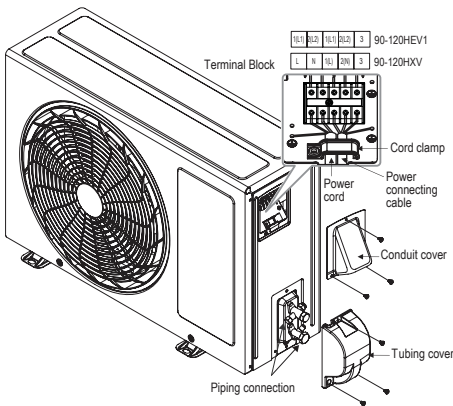
Figure 38: LSU90-120HEV1, LSU90-120HXV Outdoor Unit Connection Cover Removal.
