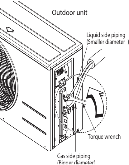
Figure 43: LSU180HEV1 Outdoor Unit Piping Connection.
