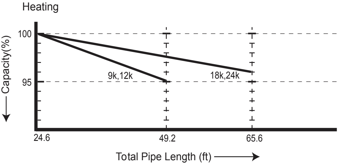
Figure 18: LS090-240HEV1 Heating Coefficient Factor.
