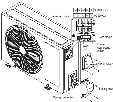
Figure 38: LSU90-120HEV1, LSU90-120HXV Outdoor Unit Connection Cover Removal.
