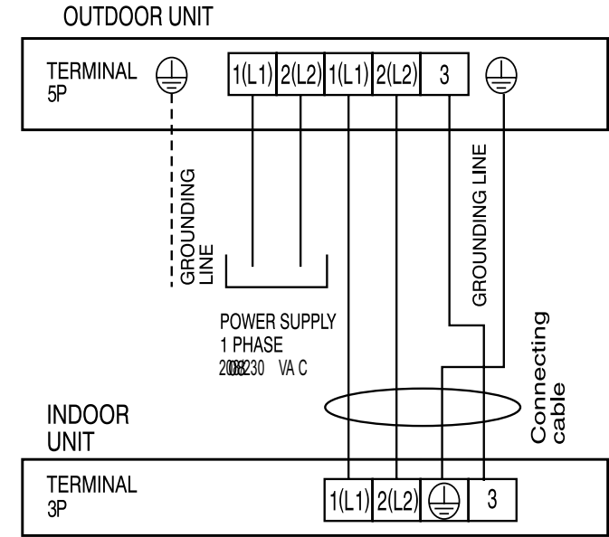
Figure 50: Terminal Block Wiring Diagram LS090HEV1 LS090HEV1
