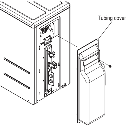
Figure 39: LSU180HEV1 Outdoor Unit Connection Cover Removal.
