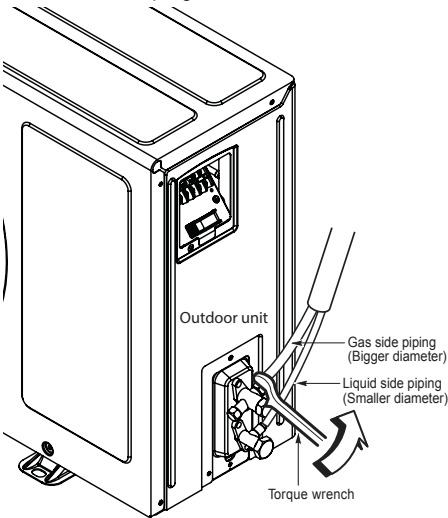
Figure 42: LSU90-120HEV1, LSU90-120HXV Outdoor Unit Piping Connection.
