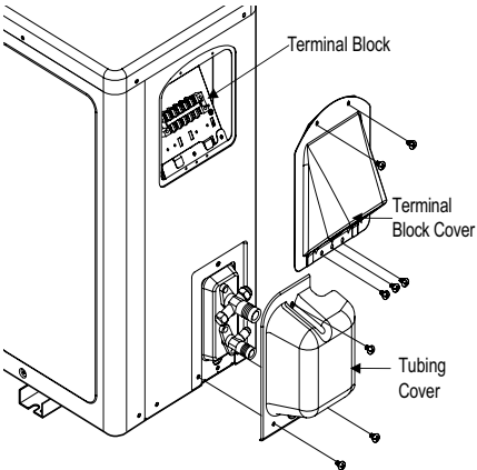
Figure 40: LSU240HEV1 Outdoor Unit Connection Cover Removal.
