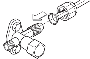
Figure 41: Pipe Attachment.
