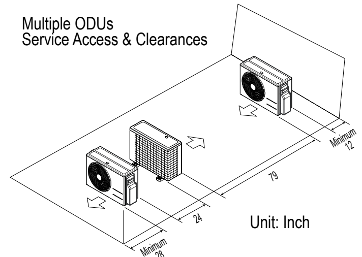
Figure 29: ODU Service Access Clearance - Multiple Units.
