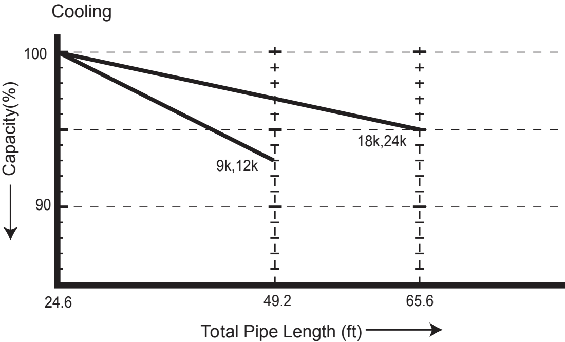
Figure 17: LS090-240HEV1 Cooling Coefficient Factor.
