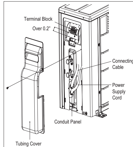
Figure 47: LSU180HEV1 Outdoor Unit Electrical Connection.
