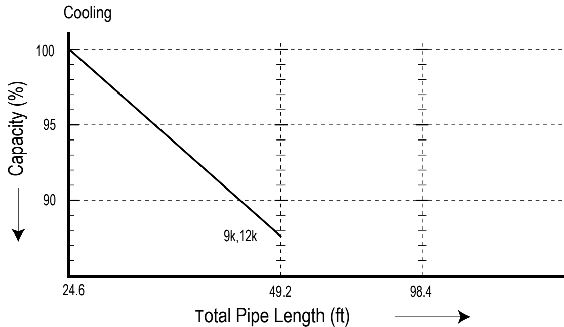
Figure 19: LS090HXV, LS120HXV Cooling Coefficient Factor.
