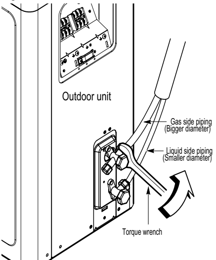
Figure 44: LSU240HEV1 Outdoor Unit Piping Connection.
