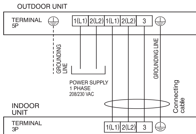
Figure 30: Terminal Block Wiring Diagram LAU090HYV1, LAU120HYV1
