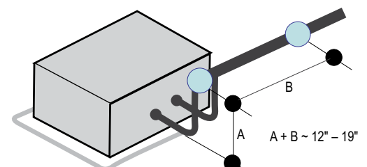
Figure 21: Pipe Support at Indoor Unit.
