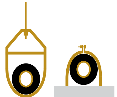
Figure 19: Pipe Hanger Details.
