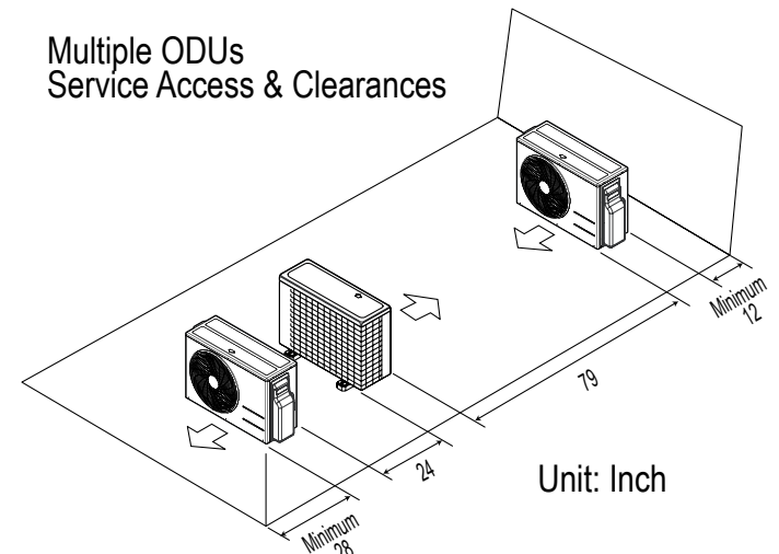
Figure 15: ODU Service Access Clearance - Multiple Units.
