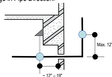
Figure 20: Typical Pipe Support Location— Change in Pipe Direction.
