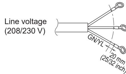
Figure 56: Power Wiring Example.
