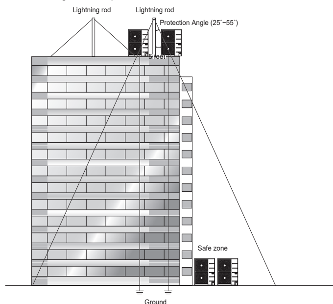
Figure 27: Lightning Protection Diagram (Outdoor Unit Appearances Differ According to Model).
