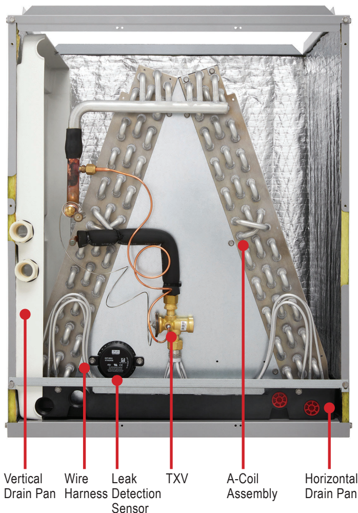
Figure 3: A-Coil Components.
