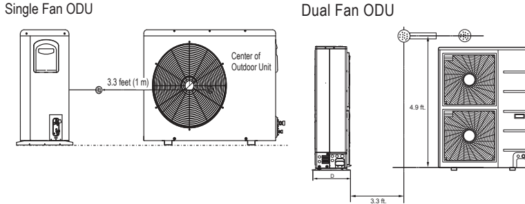
Figure 18: R32 Single-Zone CV Systems - A-Coil Outdoor Unit Sound Pressure Level Measurement Location.
