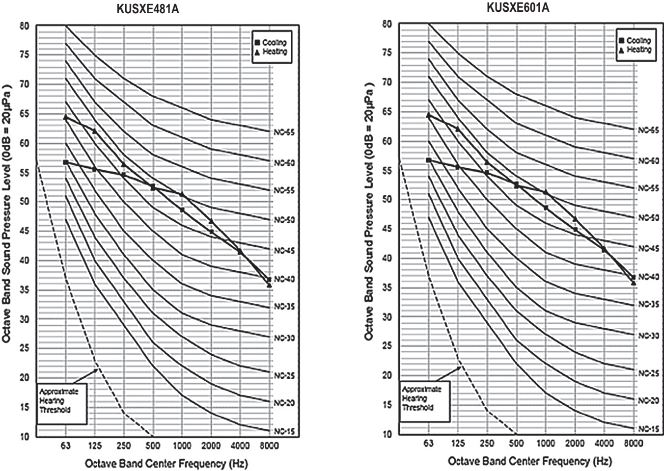
Figure 20: R32 Single-Zone CV Systems Outdoor Unit Sound Pressure Level Diagrams, continued.
