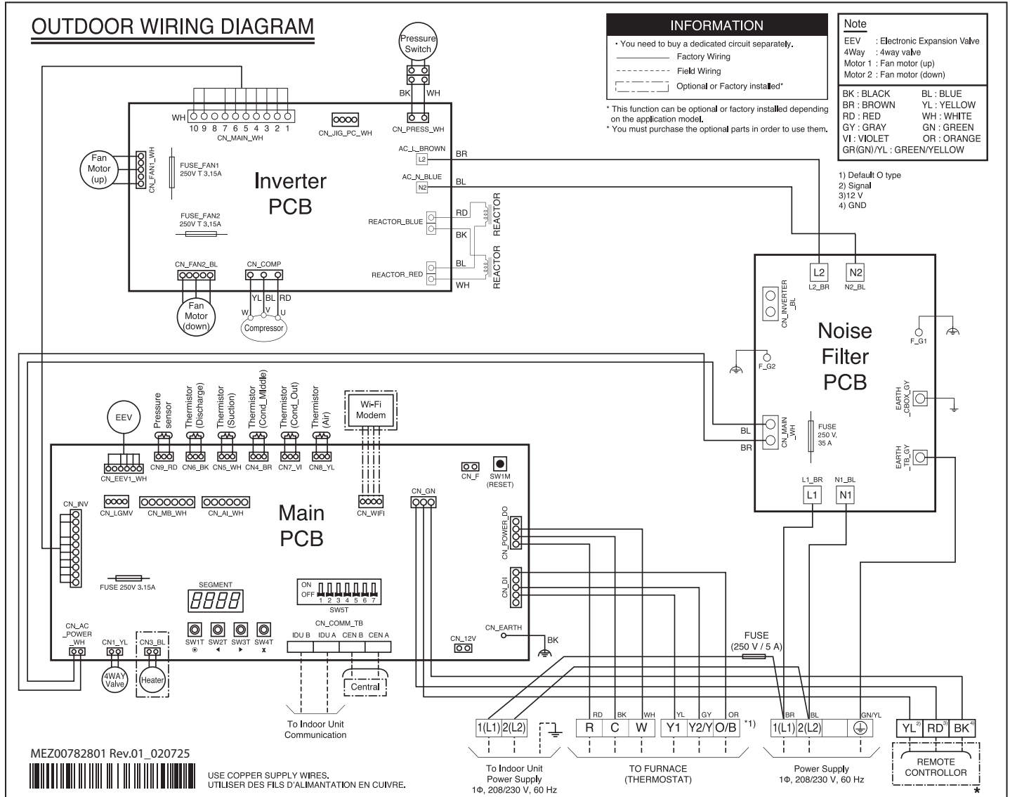
Figure 55: KUSXE481A, KUSXE601A Outdoor Units Wiring Diagram.
