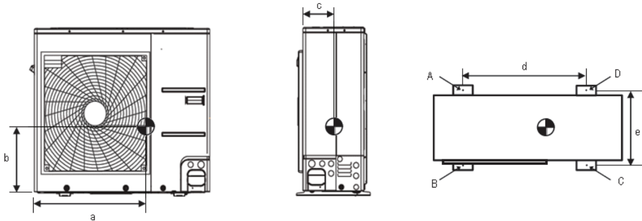
Figure 10: KUSXE241A, KUSXE361A Center of Gravity and Corner Weight Dimensions Diagram.
