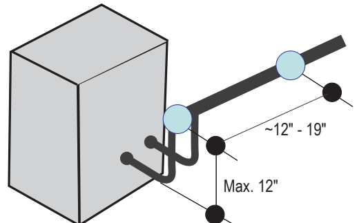
Figure 51: Pipe Support at A-Coil Unit.
