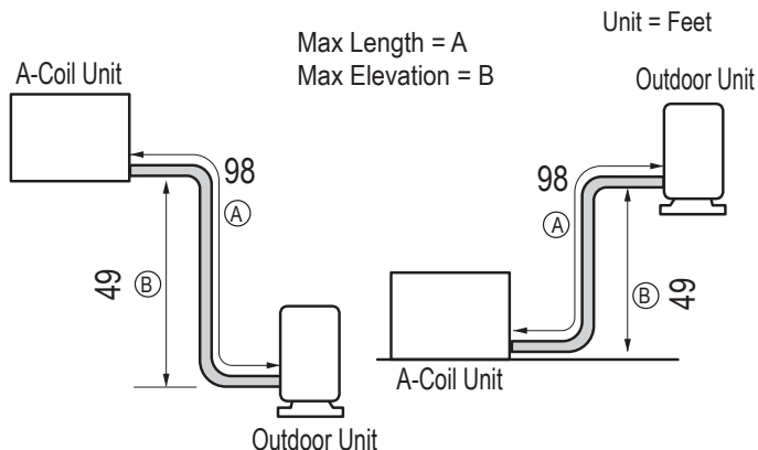
Figure 45: Typical KSSME18AA, 24BA, 36BA, 36CA System Layout.
