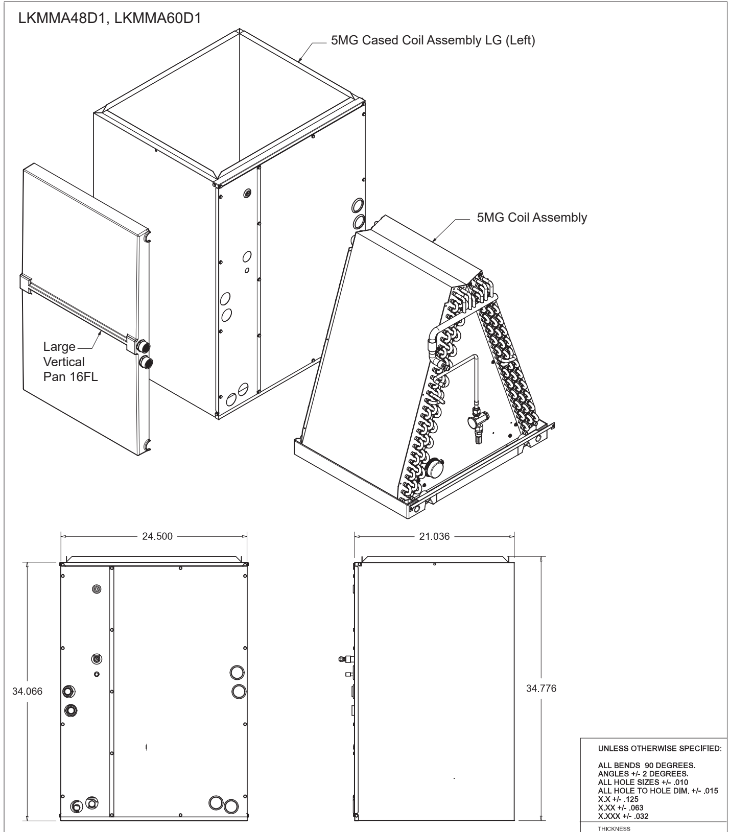
Figure 17: LKMMMA48D1, LKMMMA60D1 A-Coil Unit Dimensions.
