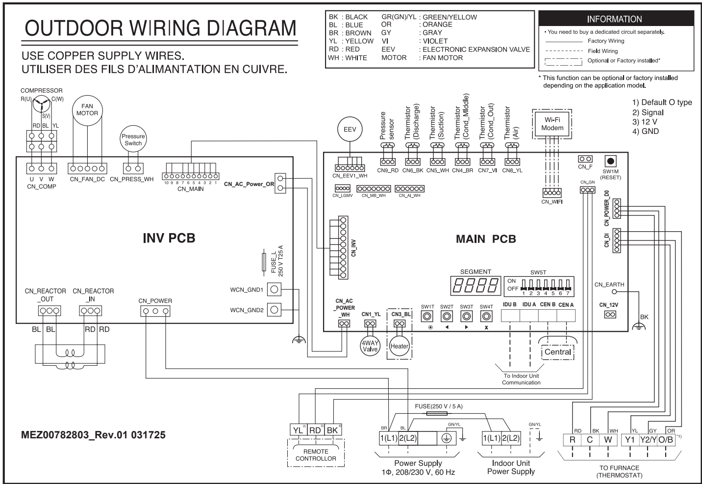
Figure 53: KUSXE241A Outdoor Units Wiring Diagram.
