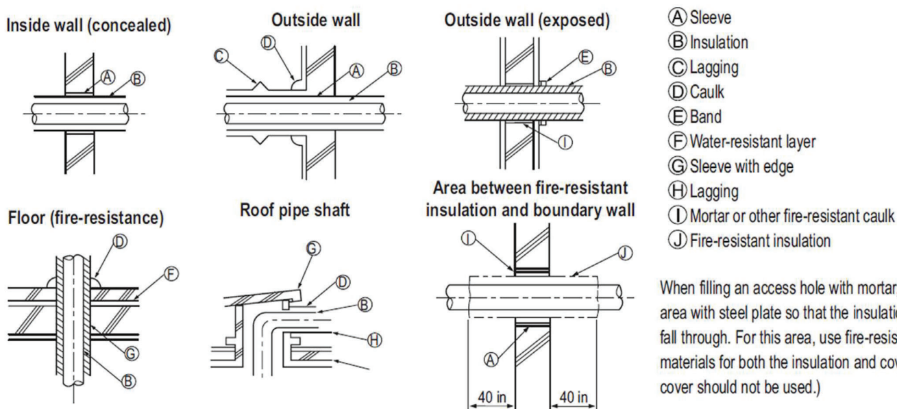
Figure 52: Pipe Sleeve Options.
