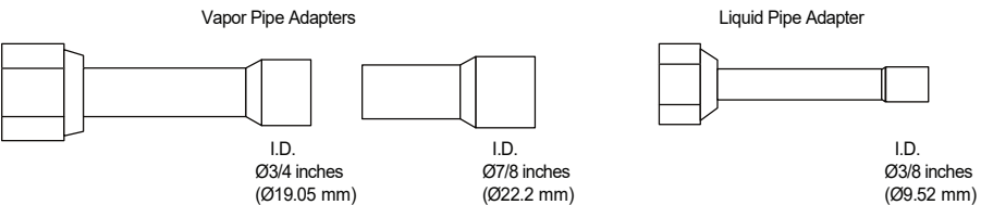
Figure 44: Adapters for A-Coil Piping.
