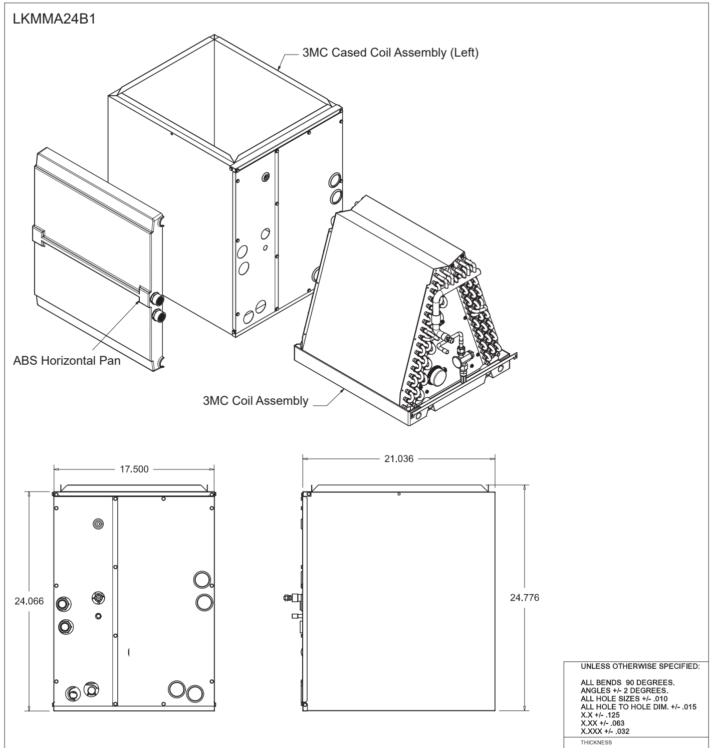
Figure 13: LKMMA24B1 A-Coil Unit Dimensions.
