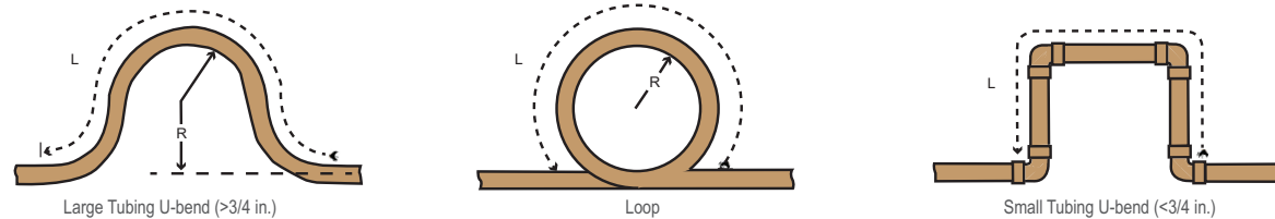
Figure 47: Coiled Expansion Loops and Offsets (Plan View).
