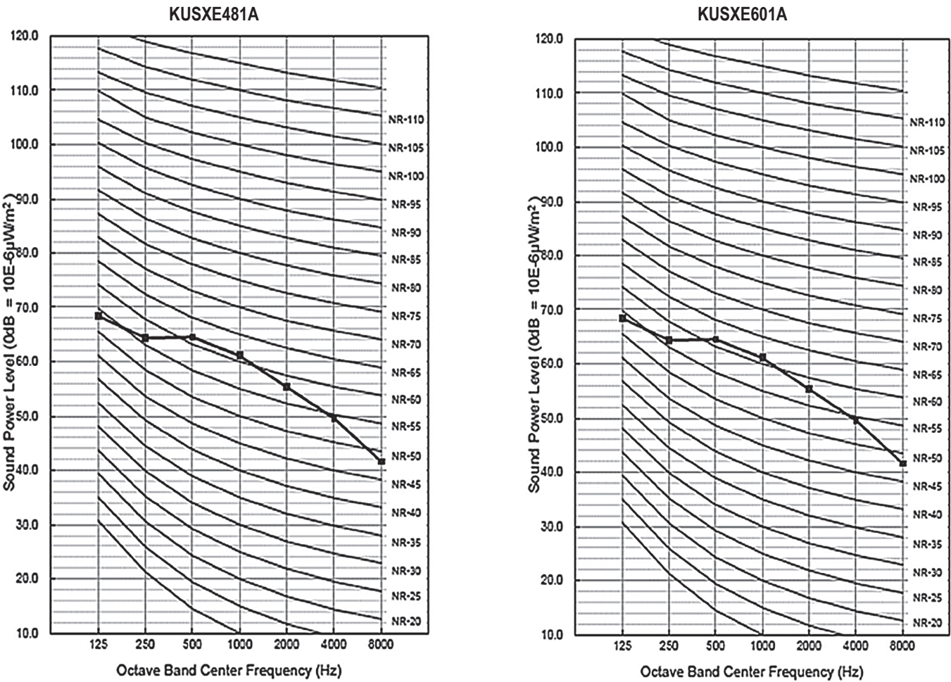
Figure 22: R32 Single-Zone CV Systems Outdoor Unit Sound Power Level Diagrams, continued.
