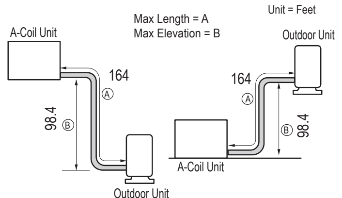
Figure 46: Typical KSSME42CA, 48CA, 48DA, 60CA, 60DA System Layout.
