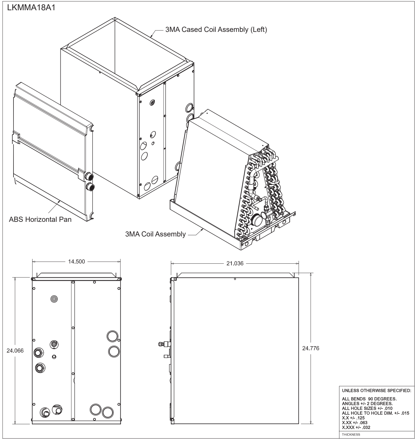
Figure 12: LKMMA18A1 A-Coil Unit Dimensions.
