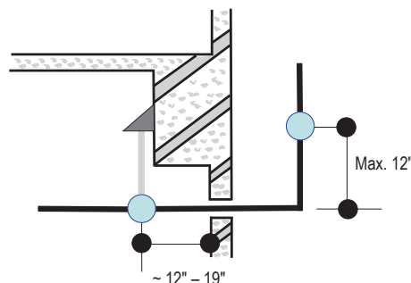
Figure 50: Typical Pipe Support Location—Change in Pipe Direction.
