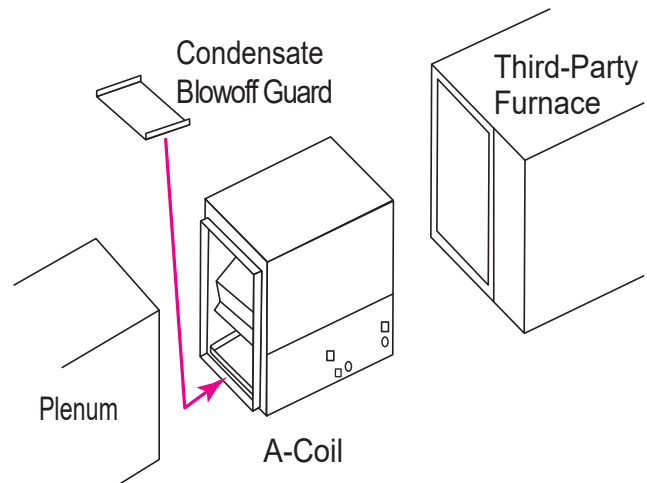
Figure 26: Horizontal Installation with Condensate Blowoff Guard.
