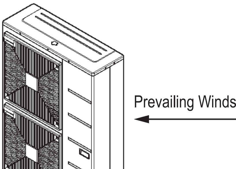
Figure 31: Oceanside Placement Using a Building as Shield, and Placement Using a Windbreak.
