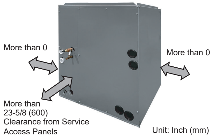
Figure 24: Example of an Upflow (Vertical) Installation.
