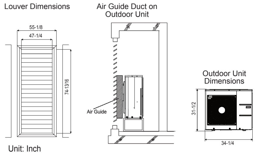
Figure 39: Example of Installing Outdoor Unit Indoors.
