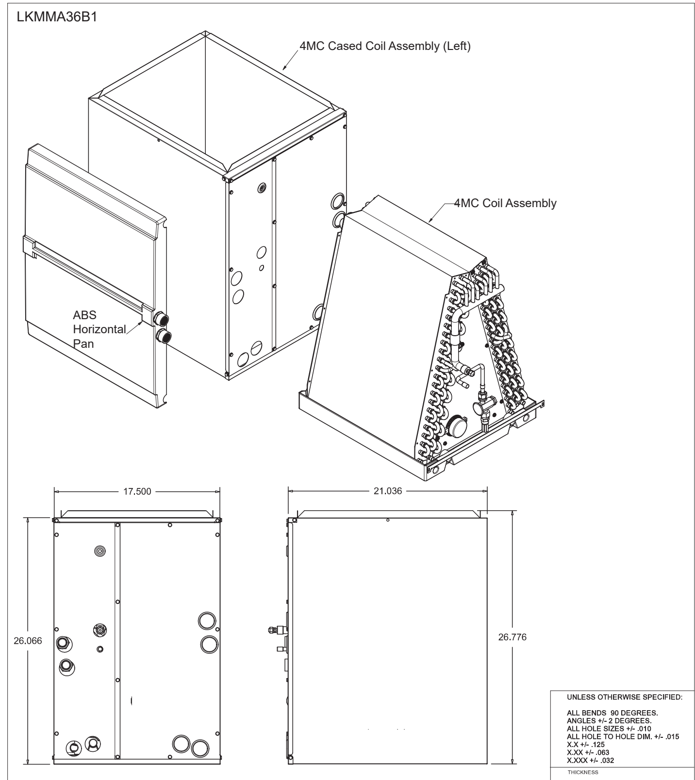
Figure 14: LKMMA36B1 A-Coil Unit Dimensions.
