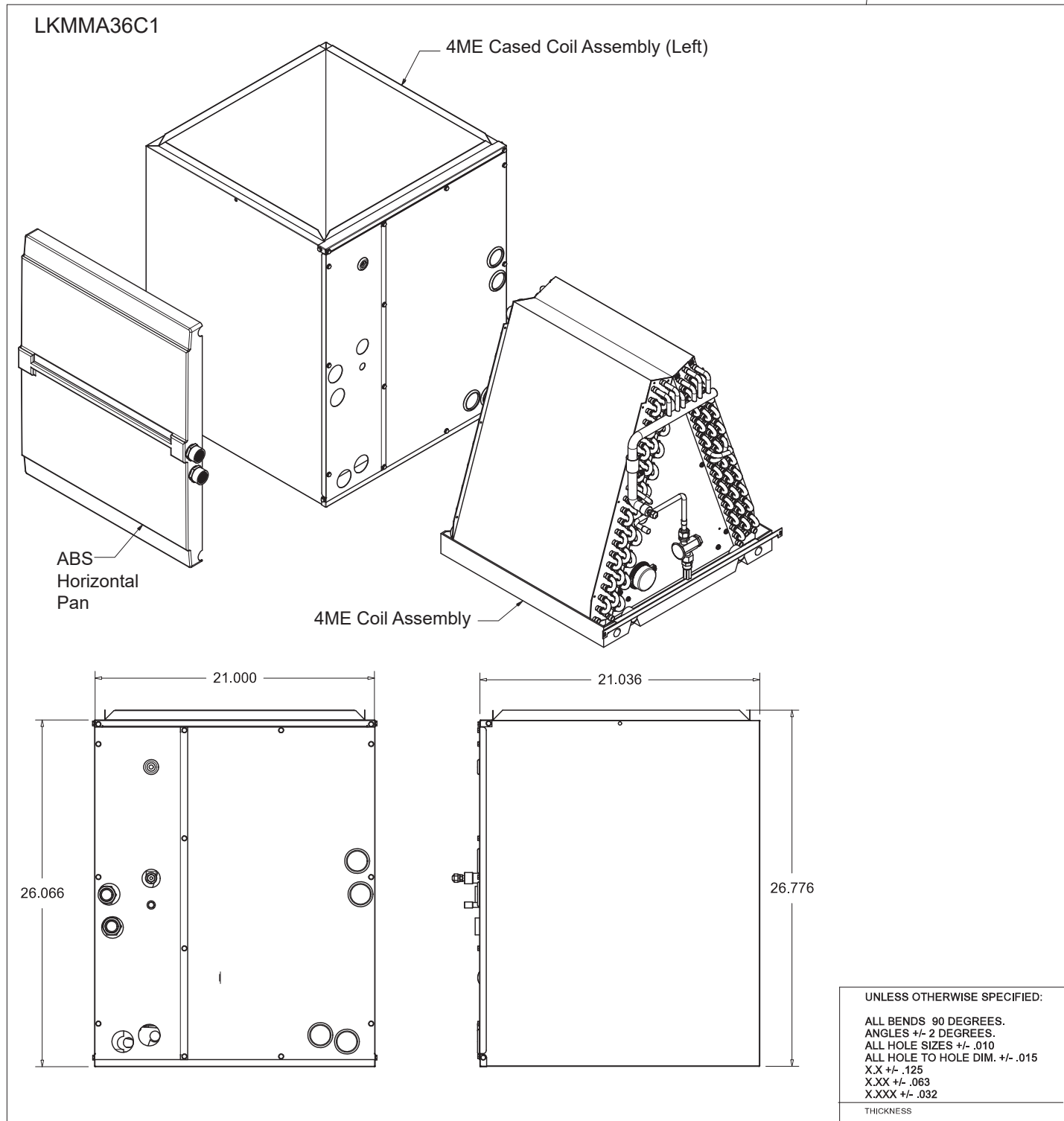
Figure 15: LKMA36C1 A-Coil Unit Dimensions.
