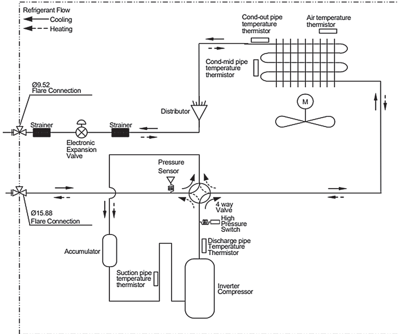
Figure 40: KUSXE241A Refrigerant Flow Diagram.
