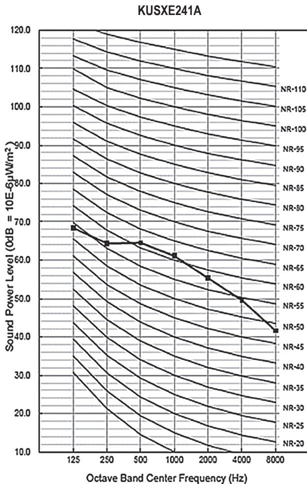
Figure 19: R32 Single-Zone CV Systems Outdoor Unit Sound Pressure Level Diagrams.
