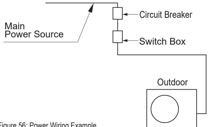
Figure 56: Power Wiring Example.
