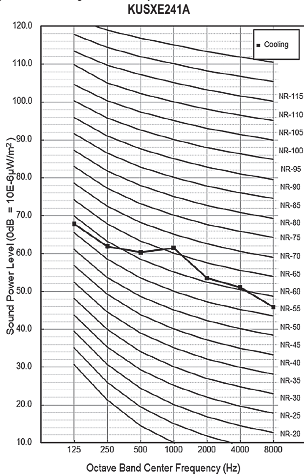
Figure 21: R32 Single-Zone CV Systems Outdoor Unit Sound Power Level Diagrams.
