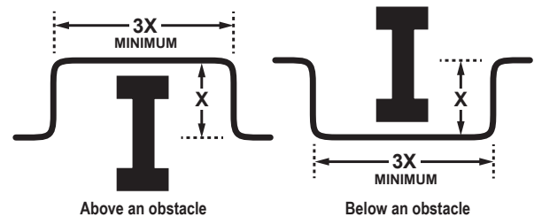
Figure 48: Installing Piping Above and Below an Obstacle.
