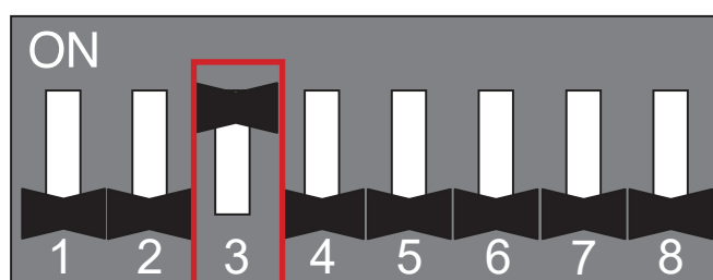
Figure 62: SW-01 DIP Switch Heat Pump Communication Kit Setting for A-Coil / Third-Party Furnace.
