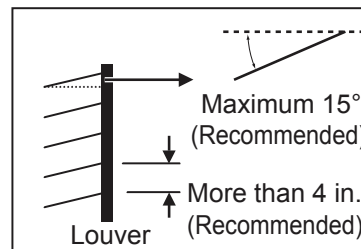
Figure 34: Louver Recommendations.
