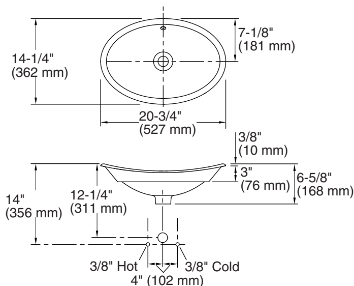
Standard Installation
