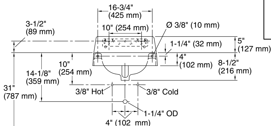
Standard Installation
