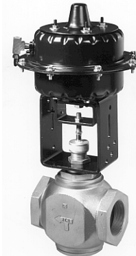
MP82 Series Pneumatic Actuator Mounted on VG7443 Brass Globe Valve
