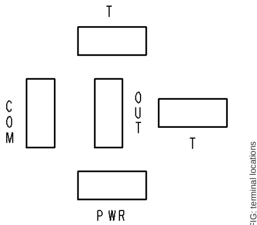
Figure 2: Terminal Locations
