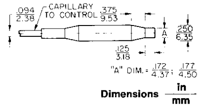
Fig. 5 — Drawing illustrating 1/4" section with reduced diameter end.
