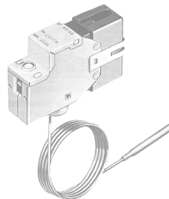
Fig. 1 -- Single function control. Optional insulated terminal cover is shown.
