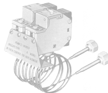
Fig. 2 -- Low pressure and high pressure controls mounted on a common bracket (Series P21).
