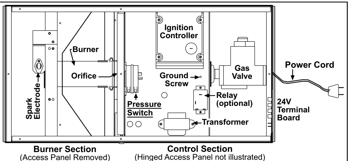
Bottom View with Access Panels Removed
