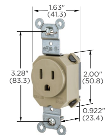
SNAP5261I
