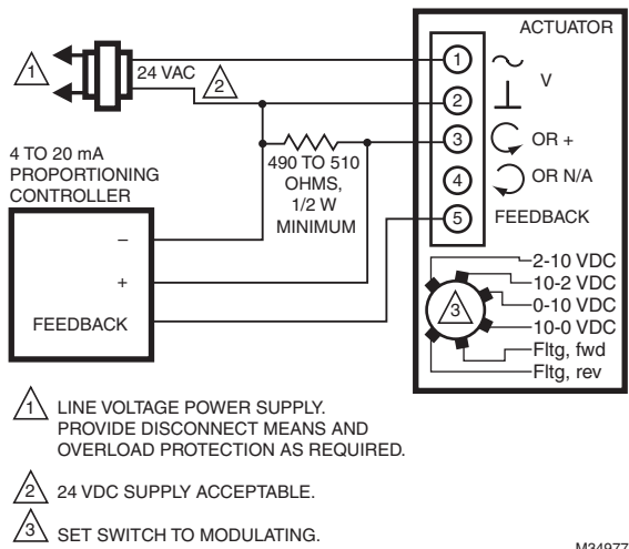
Fig. 14. MS7505 with Proportioning Controllers (Modulating mode setting).
