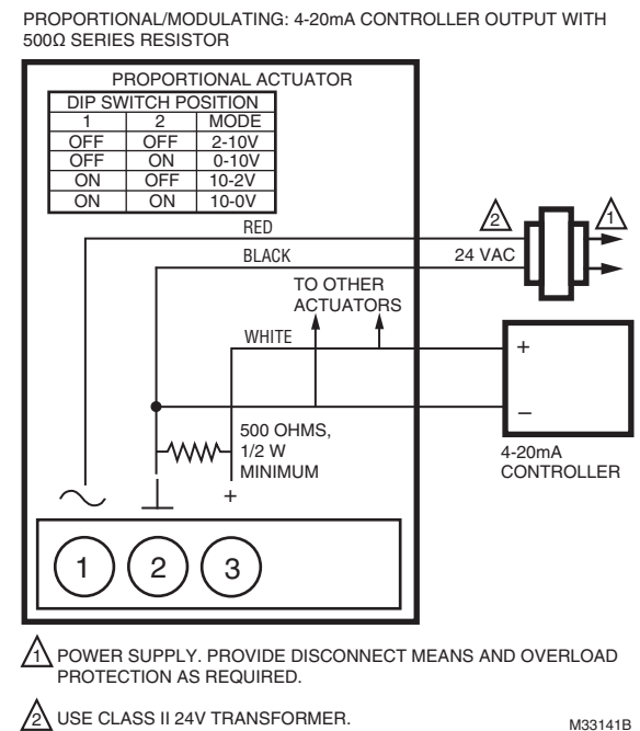
Fig. 19. MVN713 with 4-20mA Control.
