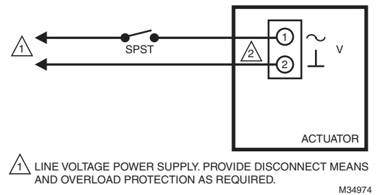
Fig. 10. MS8105 with On/Off Control.
