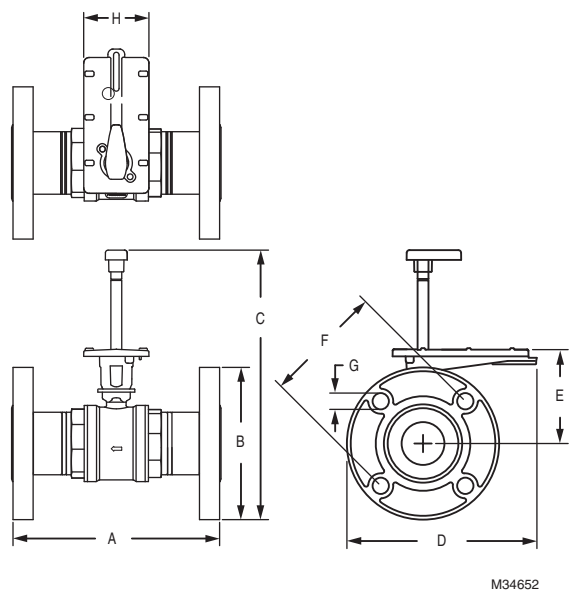
Fig. 1. 2-way 2-1/2" & 3" valve dimensions
