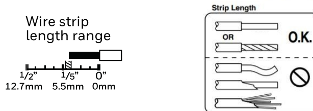
Fig. 7 Wire Strip Length
