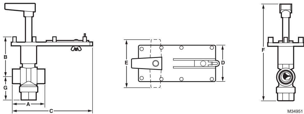
Fig. 6. 3-way ball valve dimensions for models with MN and MS actuators. See Table 8.
