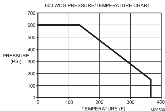
Fig. 10. Pressure derating curve.
