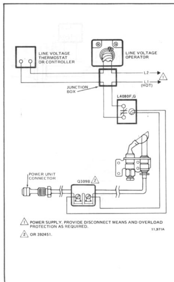
FIG. 10—L4080F,G TYPICAL WIRING HOOKUP FOR LINE VOLTAGE SYSTEMS.
