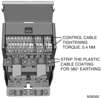
Fig. 22. Install the control cables. MI1 - MI3.
