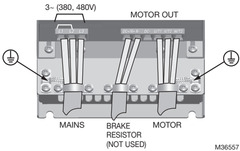
Fig. 17. SmartVFD HVAC2 power connections, MI5.
