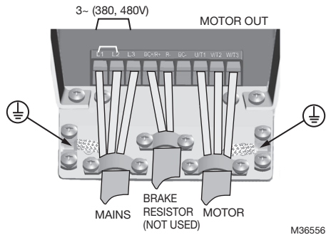
Fig. 16. SmartVFD HVAC2 power connections, MI4.
