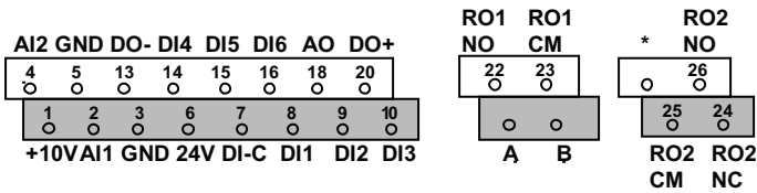
Fig. 24. SmartVFD Compact control connection terminals.
