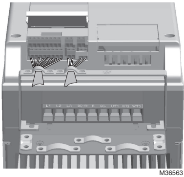
Fig. 23. Install the control cables. MI4 - MI5.
