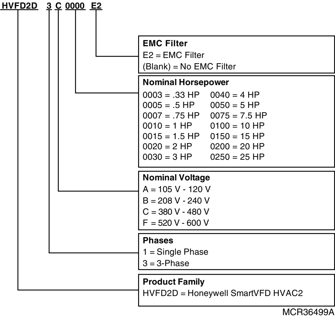
Fig. 1. SmartVFD HVAC2 type designation code.
