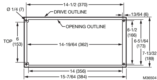
Fig. 6. Flange mounting cutout dimensions for MI4 [Unit: inches (mm)]
