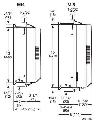
Fig. 8. Flange mounting depth dimensions for MI4 and MI5 [Unit: inches (mm)]
