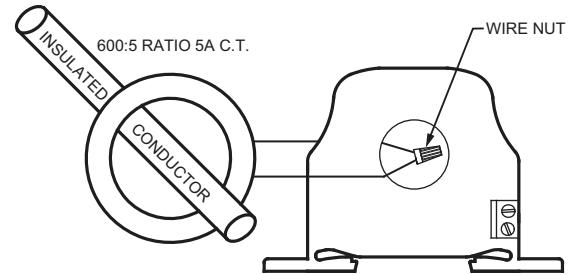
Fig. 5. Current transformer
