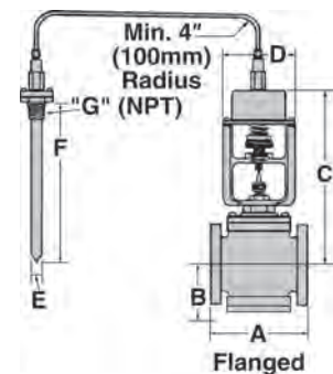
Flanged
