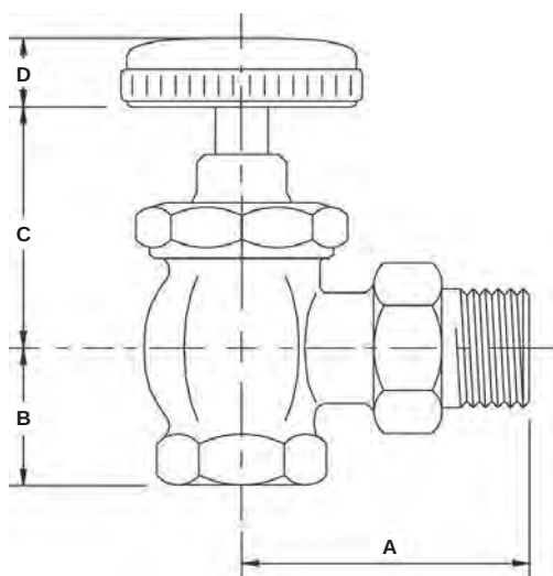
Angle Pattern
