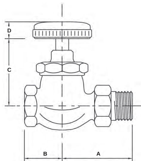
Straight Pattern
