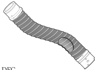
DFC Double-Wall Flexible Gas Vent Segment
