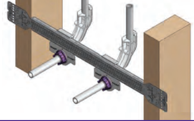
PEX 1/2" Solution Sink
