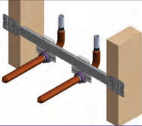
Copper to PEX 1/2" Solution Sink
