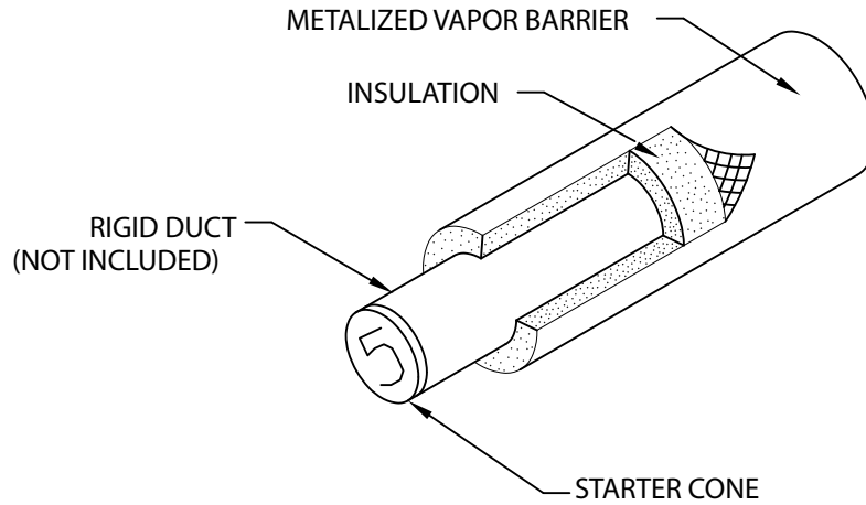
SLEEVE IS SHOWN INSTALLED
