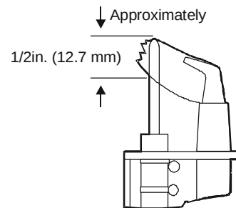
Figure 2: Flame Position
