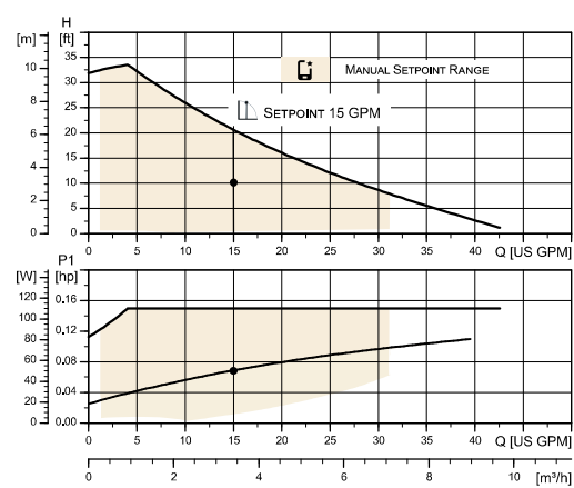
Constant flow
