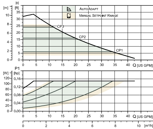
Constant pressure
