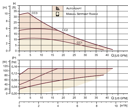
Constant curve
