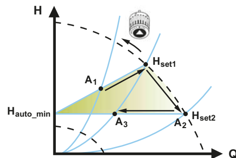
Fig. 15 AUTO_{ADAPT} control
