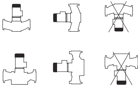
Fig. 11 Installation
