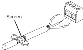
Fig. 16 External start/stop cable connection of TPE
