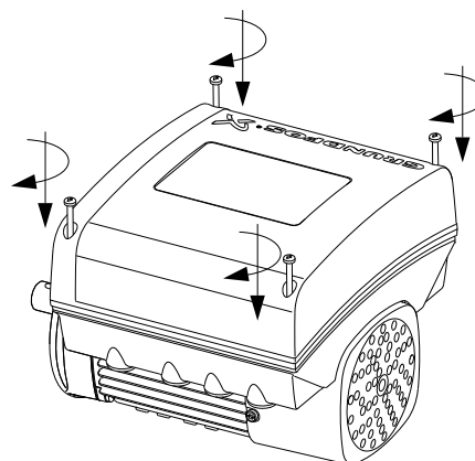
Fig. 49 Fitting the terminal box cover
