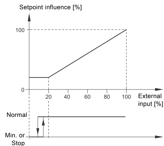
Fig. 37 "Linear with Stop" and "Linear with Min."
