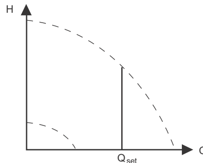
Fig. 29 Constant flow rate
