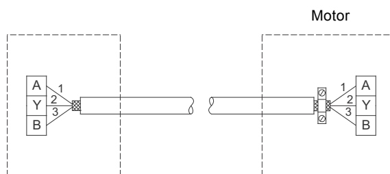
Fig. 11 Connection with screened 3-core cable
