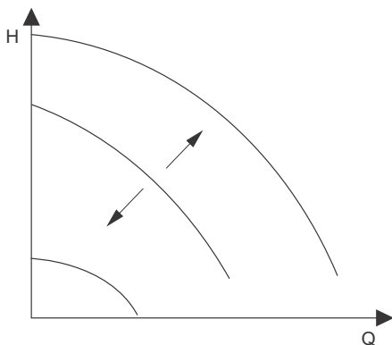
Fig. 33 Constant curve
