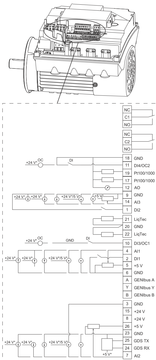
Fig. 9 Connection terminals, FM 300 (option)
