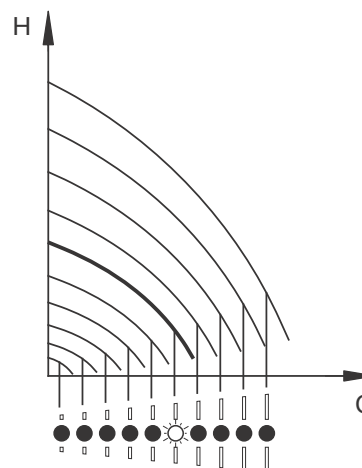
Fig. 16 Pump in constant-curve control mode
