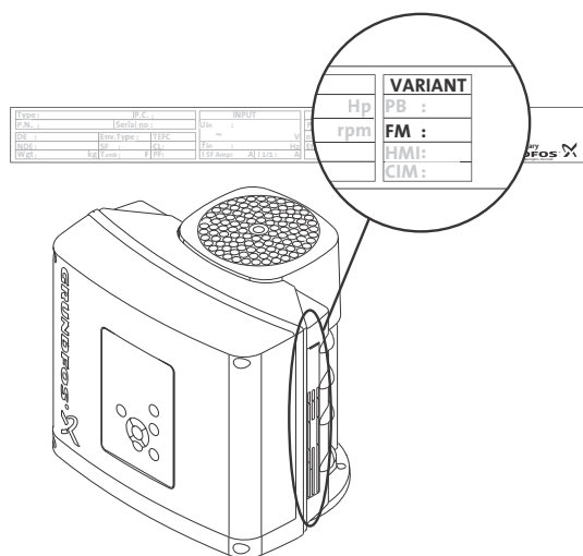
Fig. 8 Identification of functional module
