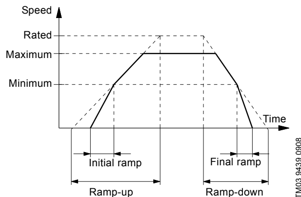
Fig. 43 Ramp-up and ramp-down
