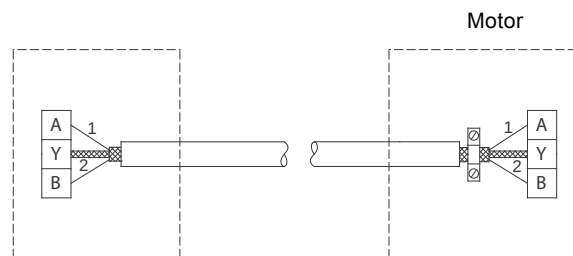
Fig. 12 Connection with screened 2-core cable
