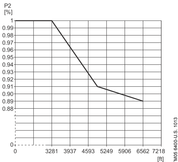
Fig. 13 Derating of motor output power (P2) in relation to altitude above sea level
