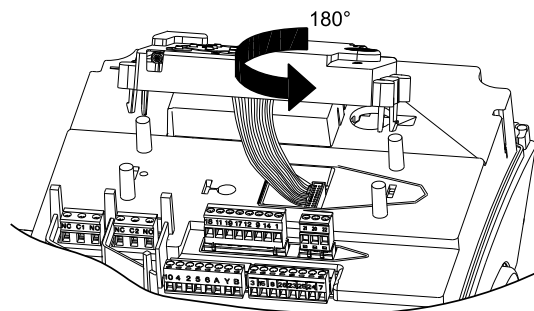
Fig. 47 Turning the plastic cover
