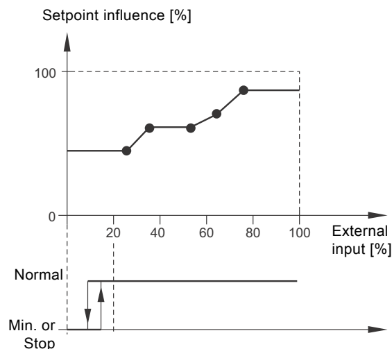
Fig. 41 Influence table with Stop at Min.
