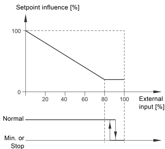
Fig. 39 "Inverse with Stop" and "Inverse with Min."
