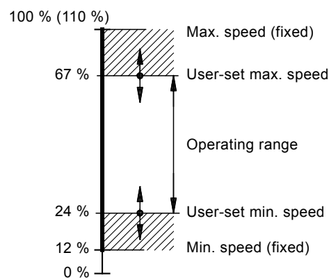
Fig. 34 Example of min. and max. settings
