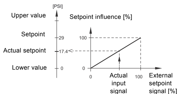
Fig. 35 Example of setpoint influence
