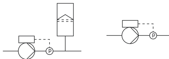
Fig. 22 Constant pressure
