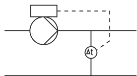
Fig. 28 Constant differential temperature
