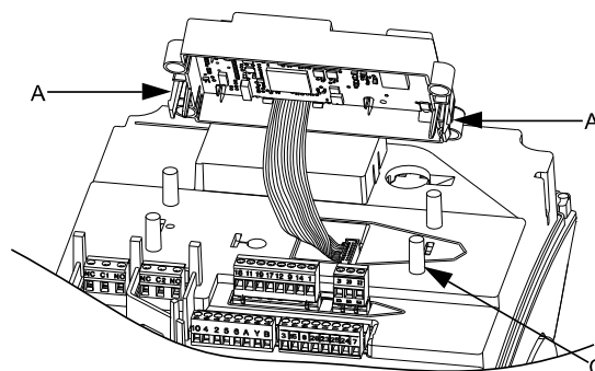
Fig. 48 Re-positioning the plastic cover
