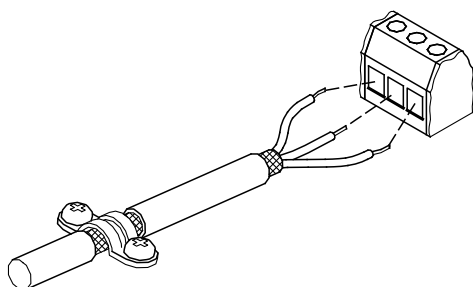
Fig. 10 Stripped cable with screen and wire connections
