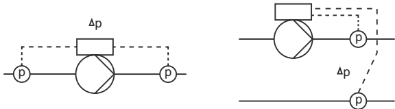
Fig. 26 Constant differential pressure
