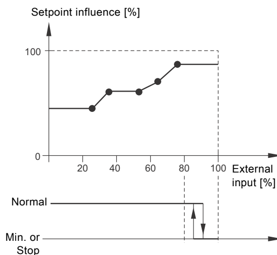
Fig. 42 Influence table with Stop at Max.
