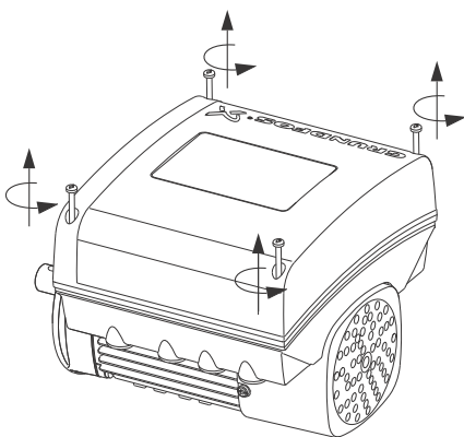
Fig. 44 Loosening the screws
