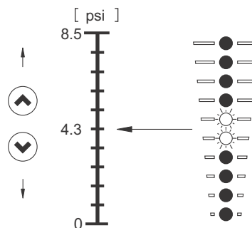
Fig. 15 Setpoint set to 4.3 psi (3 m), differential-pressure control
