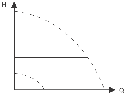
Fig. 25 Constant differential pressure
