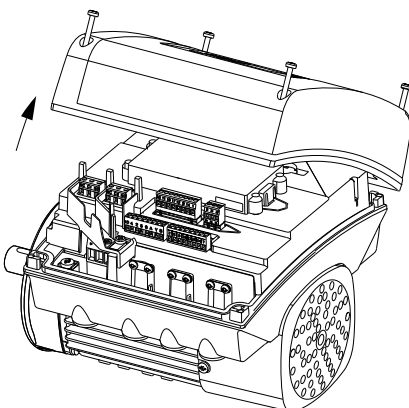
Fig. 45 Removing the terminal box cover
