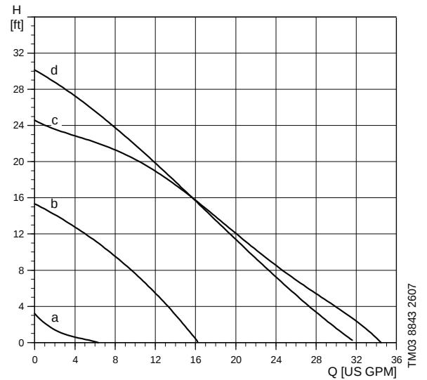
Fig. 5 Family curves for variable-speed pumps
