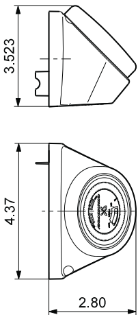
Fig. 3 Timer dimensions, current version
