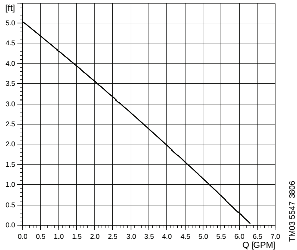
Fig. 7 Performance curve for the Comfort System
