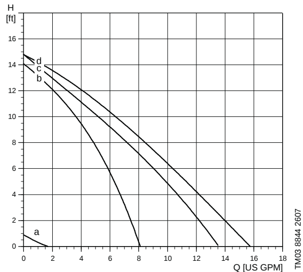
Fig. 3 Family curves for MixiMizer
