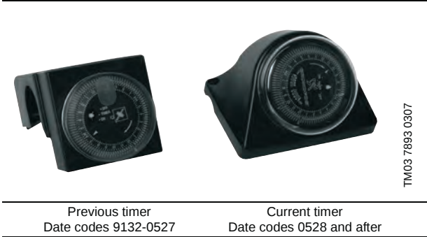
Fig. 1 UP timers
