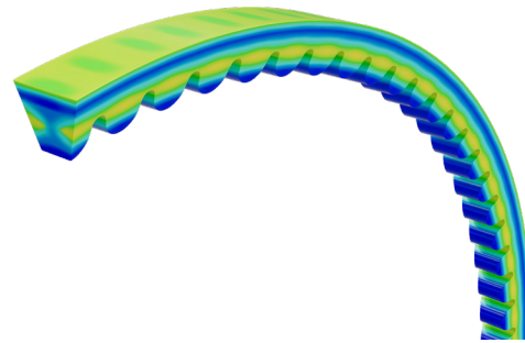
Molding notches into the belt helps reduce and spread out these stresses.
