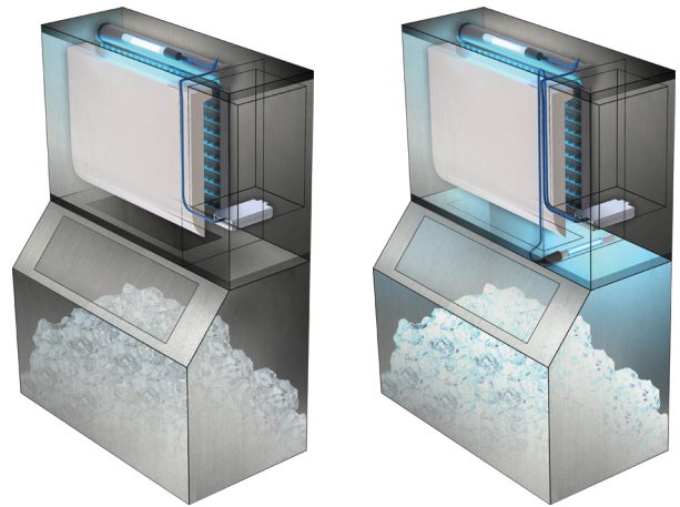
Single Lamp System: On lid between evaporator and deflector
