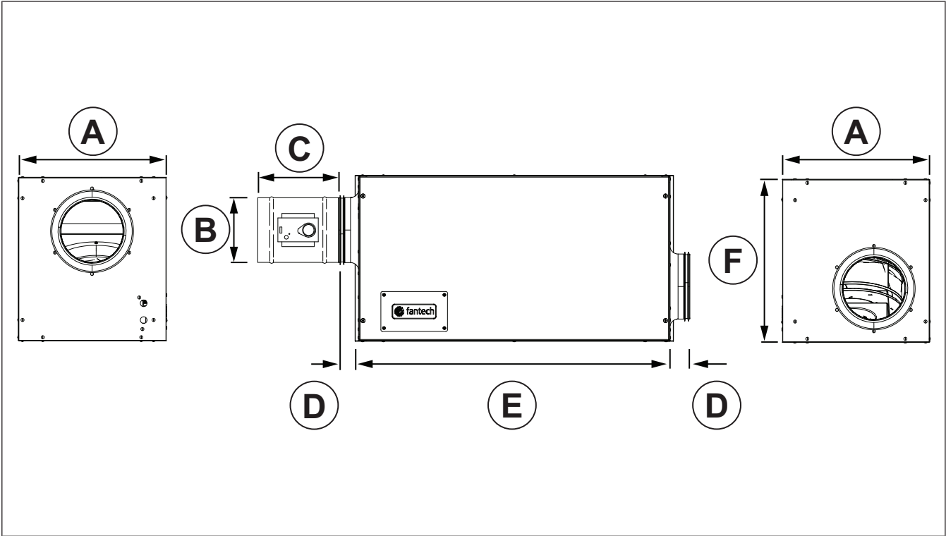
Fig. 12 MUAS Dimensions
