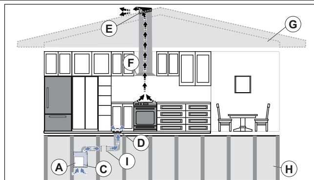
Fig. 3 Crawlspace Installation, Wall Mount — Makeup Air Shown Supplied Behind the Kick Board
