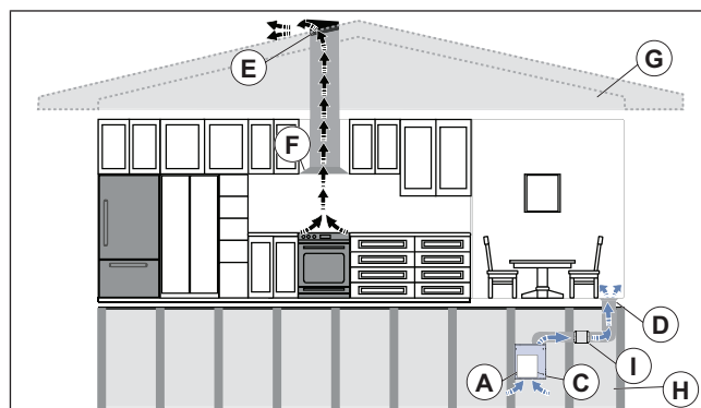
Fig. 4 Crawlspace Installation, Wall Mount — Makeup Air Shown Supplied in the Dining Room
