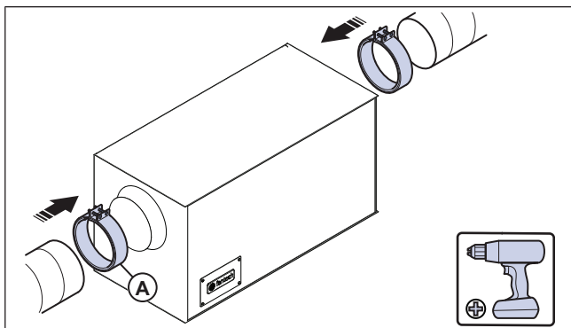
A. FC Mounting Clamps
