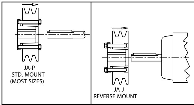
ILLUSTRATION 1B - - QD ASS'Y, FLANGE OUTBOARD
