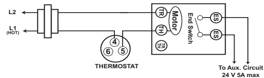
Figure-2 Typical Wiring of a PopTop to Replace a Flair or White-Rodgers 3-Wire Valve.
