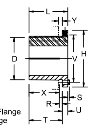
"S" & "U" BUSHINGS
