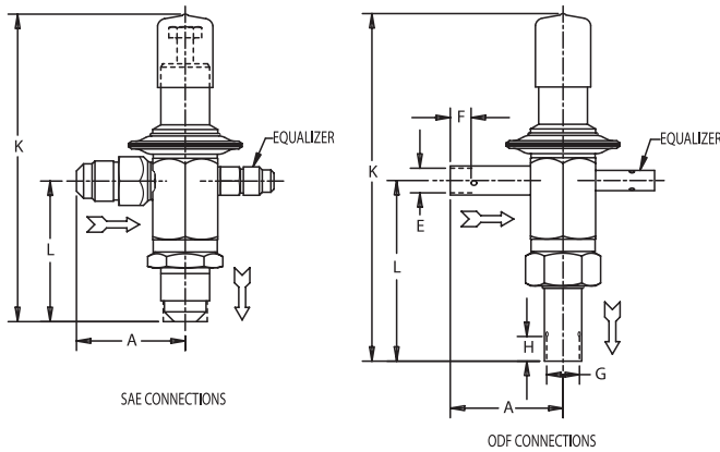
ACP Angle
