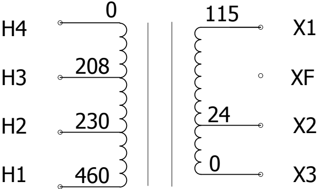
CONNECTION DIAGRAM
