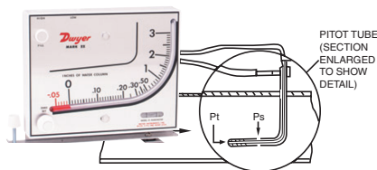
PITOT TUBE SENSES TOTAL AND STATIC PRESSURES. MANOMETER MEASURES VELOCITY PRESSURE-(DIFFERENCE BETWEEN TOTAL AND STATIC PRESSURES).
