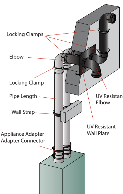
Horizontal Twin Pipe Elbow Termination
