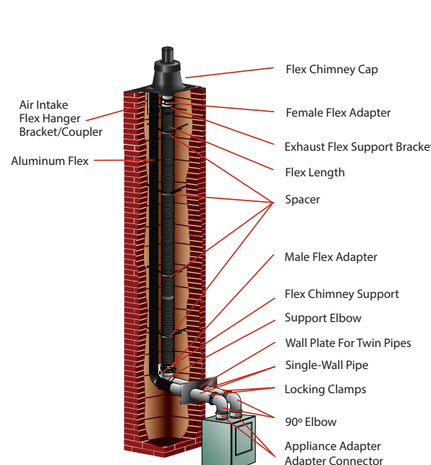
Twin Pipe with Concentric Termination
