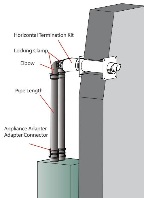
Horizontal Twin Pipe Concentric
