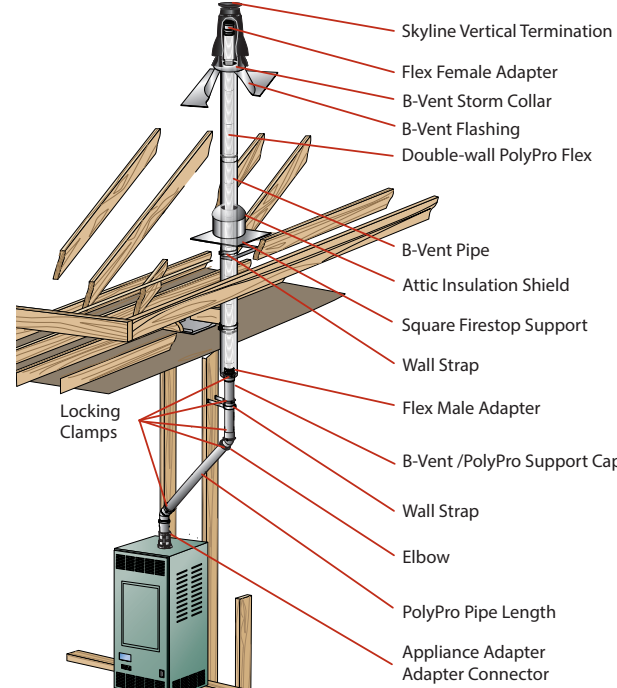
Flex Through B Vent as a Chase
