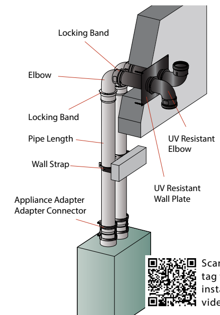
Horizontal Twin Pipe Elbow Termination
