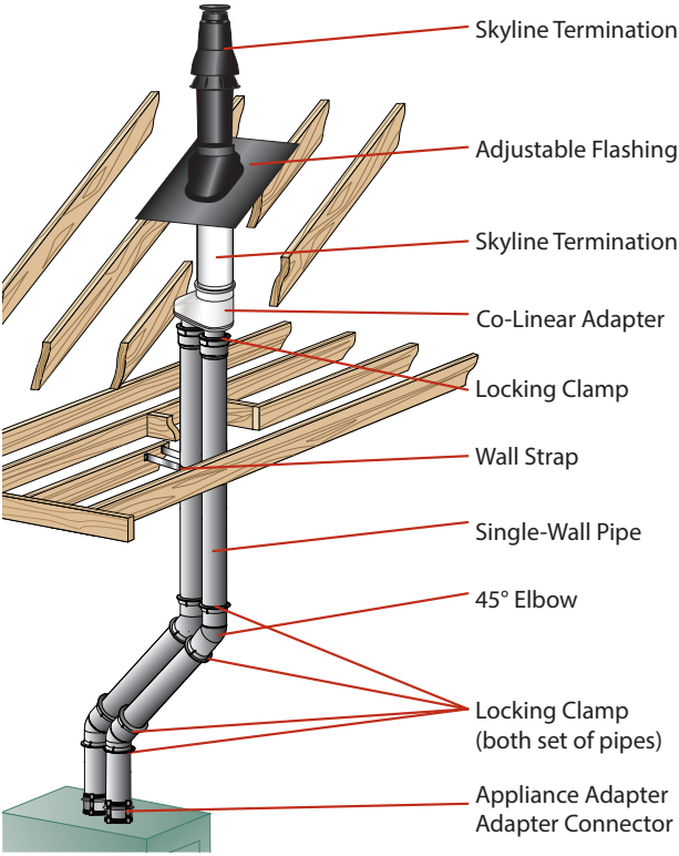
Twin Pipe with Concentric Termination
